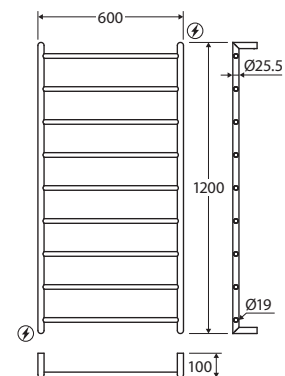
⚡ Wiring Positions
