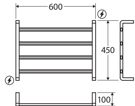
⚡ Wiring Positions
