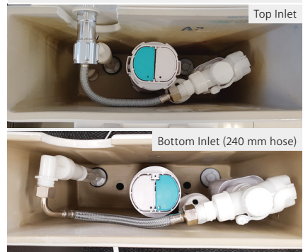
Standard R&T cistern
